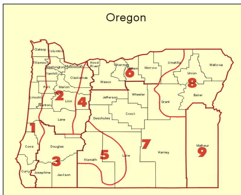
Figure DR-1 Map of Climatic Divisions
