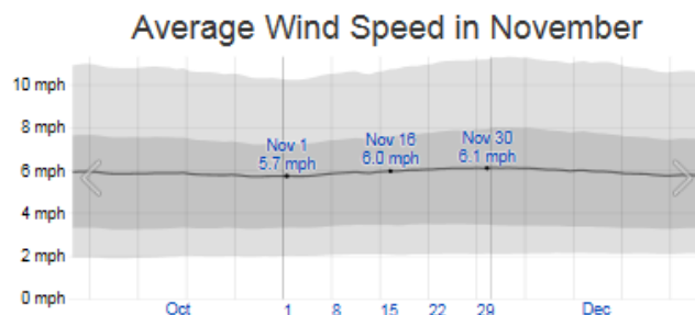
Figure C-10 Average Wind Speed in November
