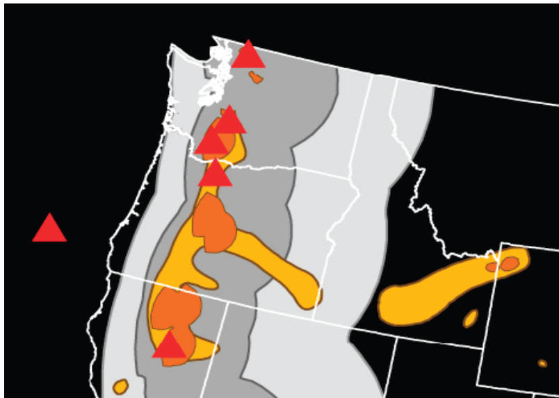
Figure VE-4 National Volcanic Hazard Map
