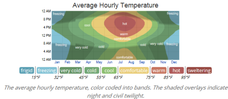
Figure C-6 Average Hourly Temperature in Ontario, Oregon
