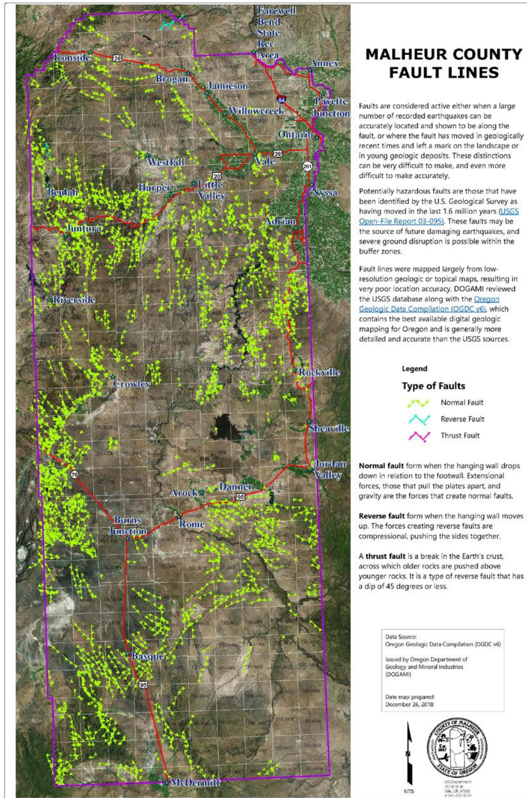
Figure EQ-7 Malheur County Fault Lines
