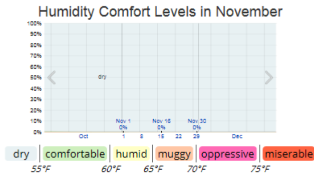
Figure C-9 Humidity Comfort Levels in November
